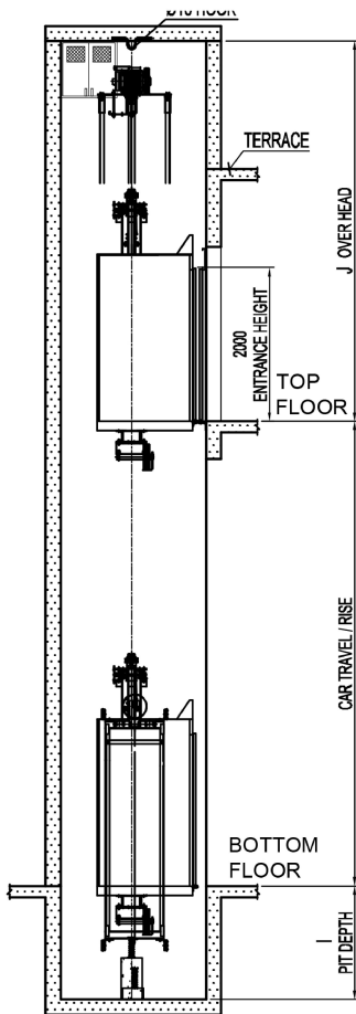
Sectional Elevation
