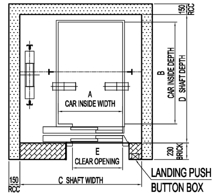
Plan Of Elevator Shaft
